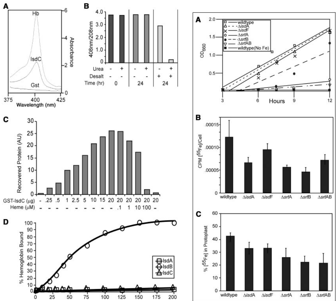
Fig. 3 (left). The isd locus encodes heme-binding proteins. (A) Spectrophotometric analysis of purified Gst-IsdC and hemoglobin (Hb) at 408 nm, the absorbance of heme. (B) Denaturation with 8 M urea, 24-hour incubation at room temperature, and desalting suggest a noncovalent interaction between heme-iron and Gst-IsdC. (C) Gst-IsdC binds heme-agarose beads in a dose-dependent manner and incubation with heme-iron abolishes this binding. (D) His-IsdB, but not Gst-IsdA or Gst-IsdC, binds human hemoglobin in a dose-dependent manner. Fig. 4 (right). S. aureus requires sortases and Isd proteins to internalize heme-iron. (A) Growth of S. aureus Newman in iron-free medium is restored when heme-iron is added. Deletion of the sortase A ( srtA ), sortase B ( srtB ), isdA , and isdF genes and their effect on the growth of mutant staphylococci in heme-iron-containing growth medium. (B) Inactivation of isdA , isdF , srtA , or srtB leads to a decrease in the amount of [ 55 Fe]heme-iron associated with cells of S. aureus as measured in scintillation counts per minute of 55 Fe. (C) Inactivation of isdA , isdF , srtA , or srtB decreased the amount of [ 55 Fe]heme that enters the staphylococcal cytoplasm.
